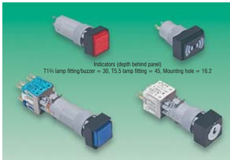
Switches (depth behind panel) T1¼ lamp fitting/key switch = 55, T5.5 lamp fitting = 70, Mounting Hole = 16.2
